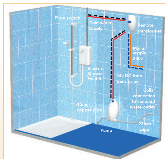
PUMP DIAGRAM
